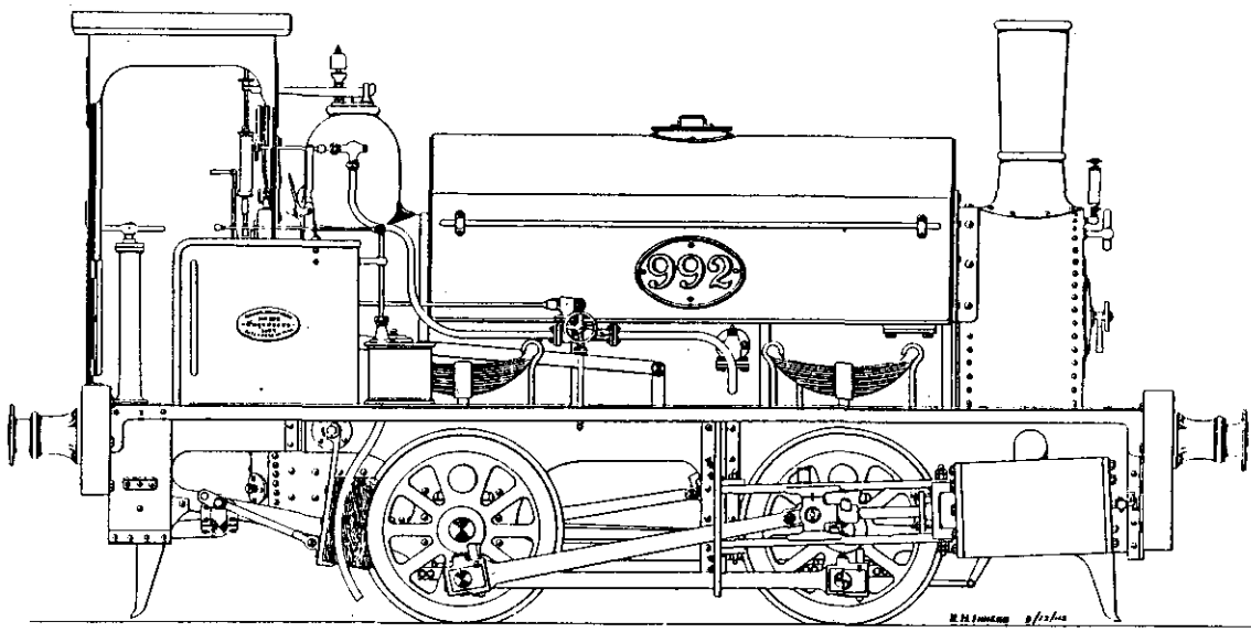
NER No. 992. a Black, Hawthorn 0-4-0ST.
